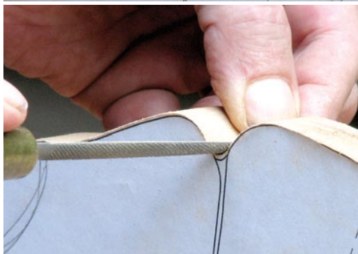
Rasp to the rescue. The flat side of this rasp removes the band-saw marks on most of the edge. The round side gets into places the flat side can't reach. Many of the finished tight curves are defined by the shape of the tool.
